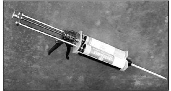
"Quick Mix" 1:1 Manual Gun
